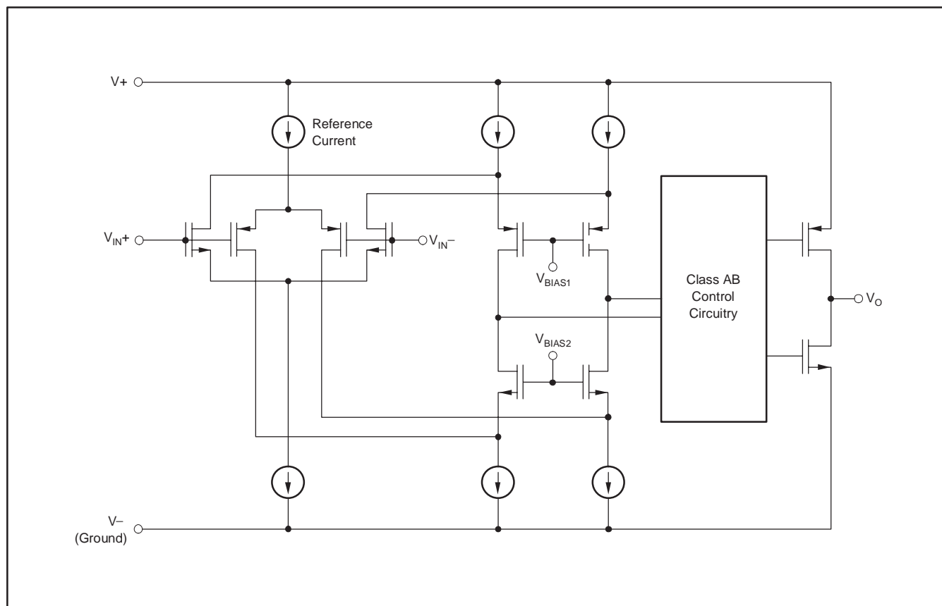
Figure 1. Simplified Schematic
