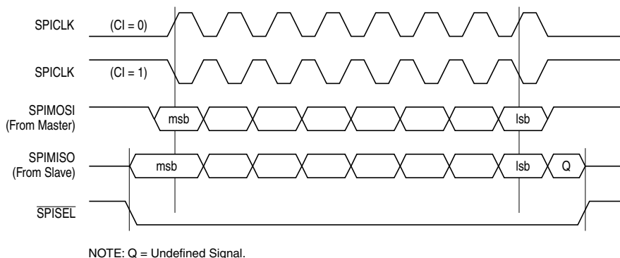
Figure 31-5. SPI Transfer Format with SPMODE[CP] = 0
