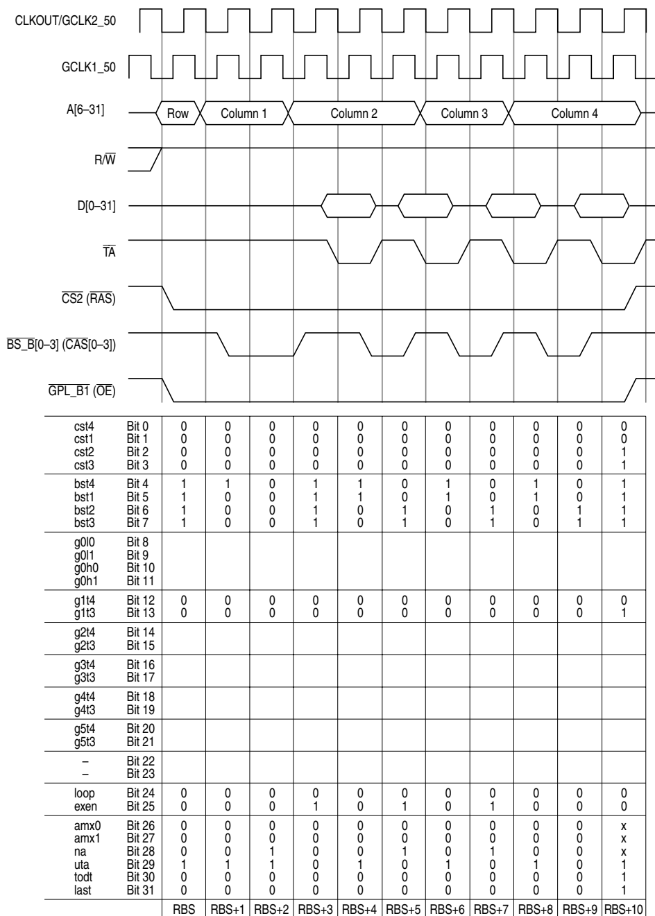
Figure 15-66. EDO DRAM Burst Read Access
