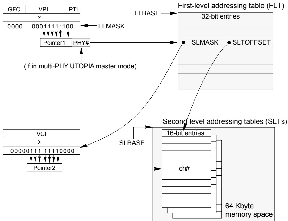
Figure 39-2. Address Compression
