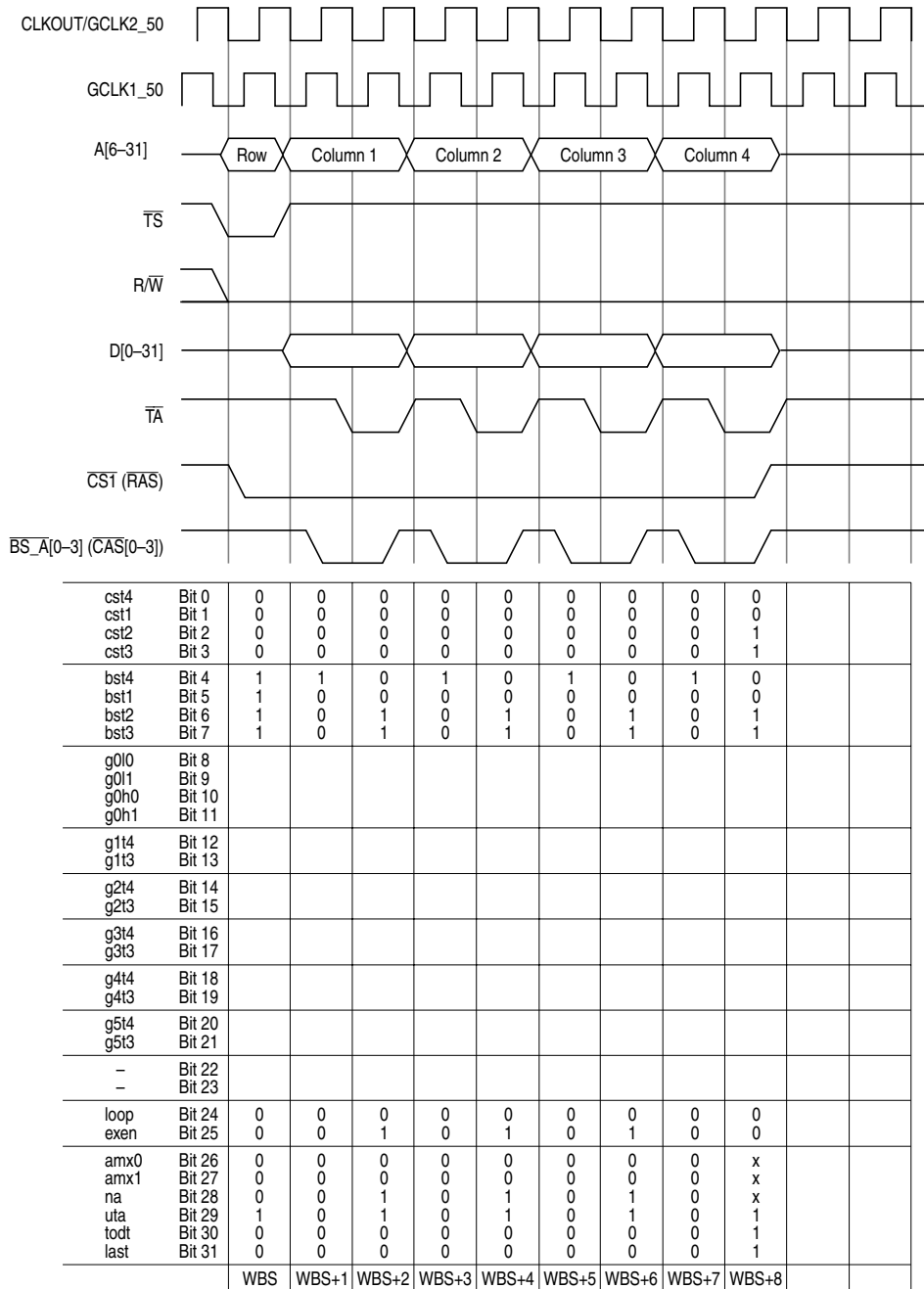
Figure 15-58. Burst Write Access to Page-Mode DRAM (No LOOP)
