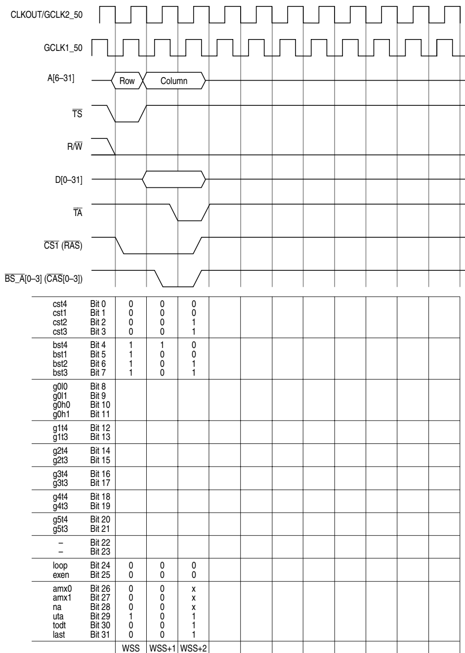
Figure 15-55. Single-Beat Write Access to Page Mode DRAM
