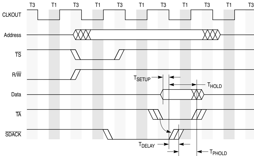
Figure 19-11. \overline{\text{SDACK}} Timing Diagram: Single-Address Peripheral Write, Internally-Generated TA
