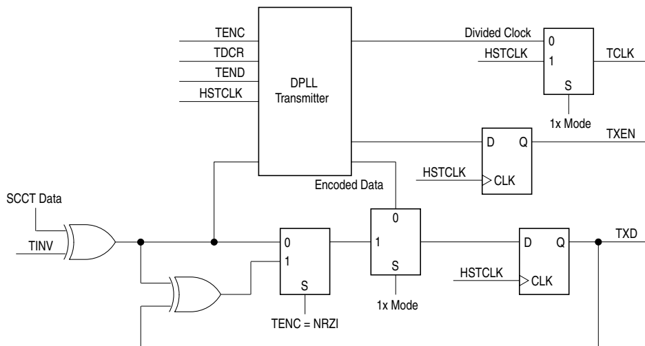
Figure 21-14. DPLL Transmitter Block Diagram
