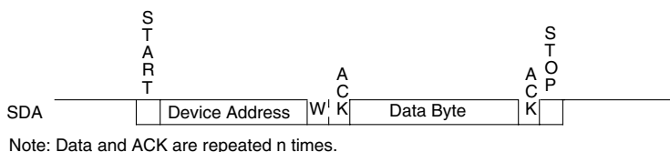
Figure 33-4. I2C Master Write Timing
