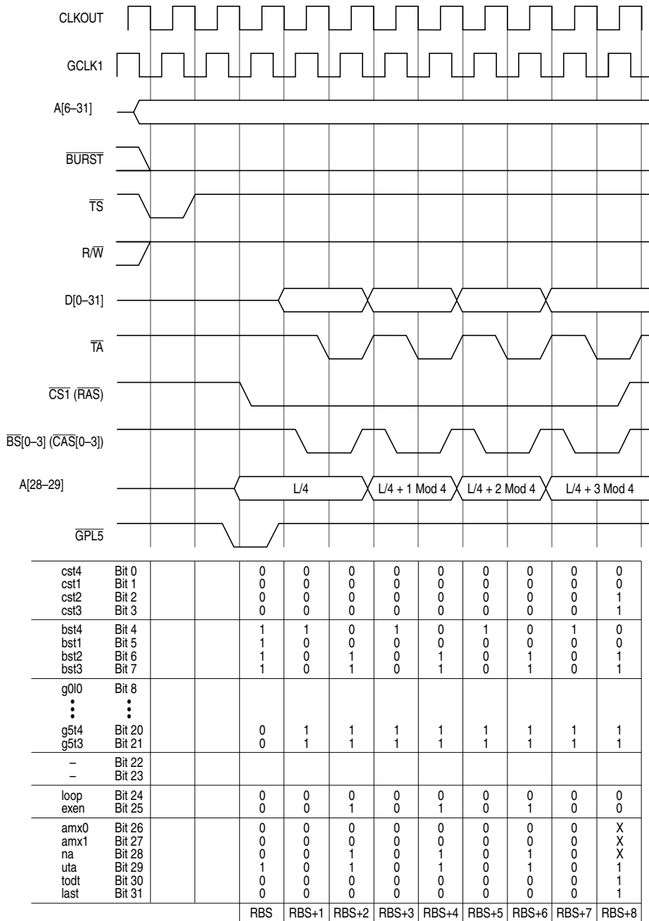
Figure 15-50. Synchronous External Master: Burst Read Access to Page Mode DRAM
