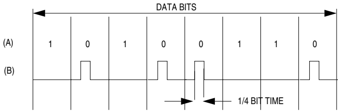
Figure 29-4. Middle-Speed IrDA Data Format
