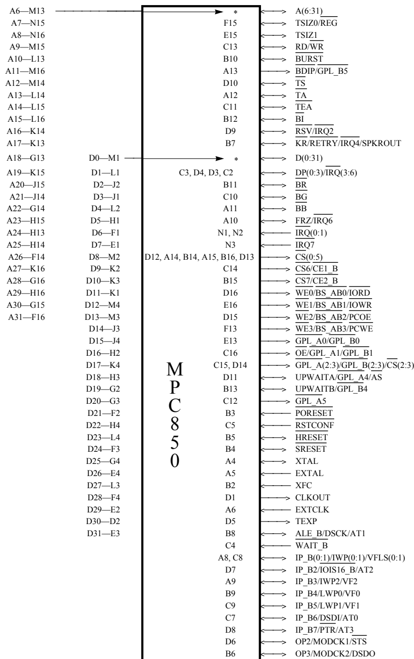
Figure 12-3. MPC850 Signals and Pin Numbers (Part 2)
