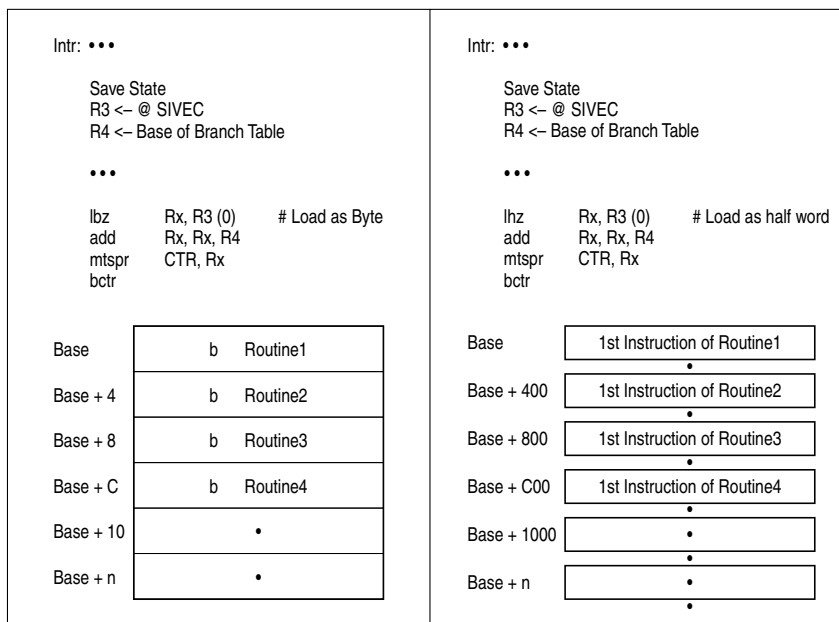
Figure 10-14. Interrupt Table Handling Example
