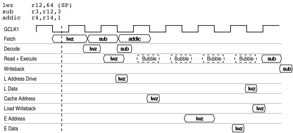
Figure 9-5. External Load Timing
