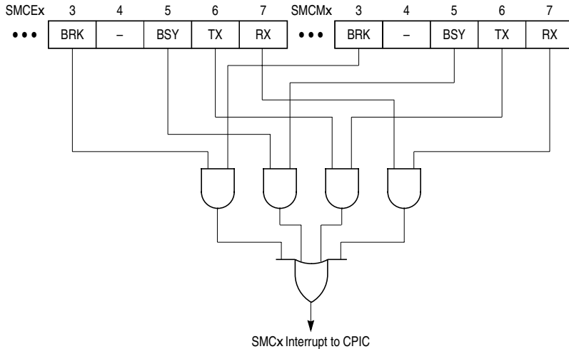
Figure 35-2. Interrupt Request Masking
