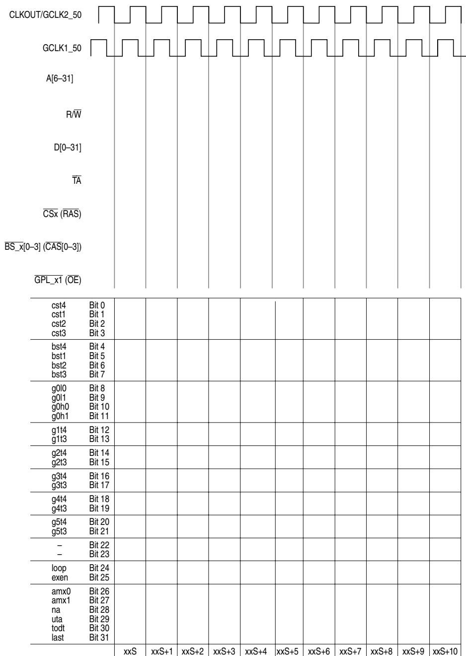
Figure 15-70. Blank Work Sheet for a UPM
