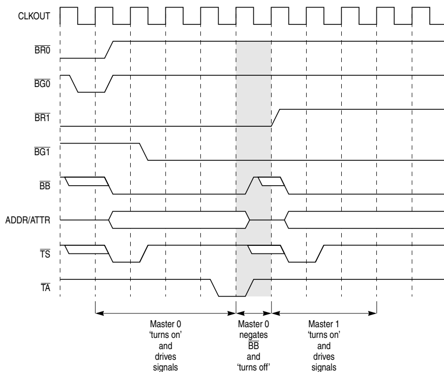
Figure 13-23. Bus Arbitration Timing Diagram
