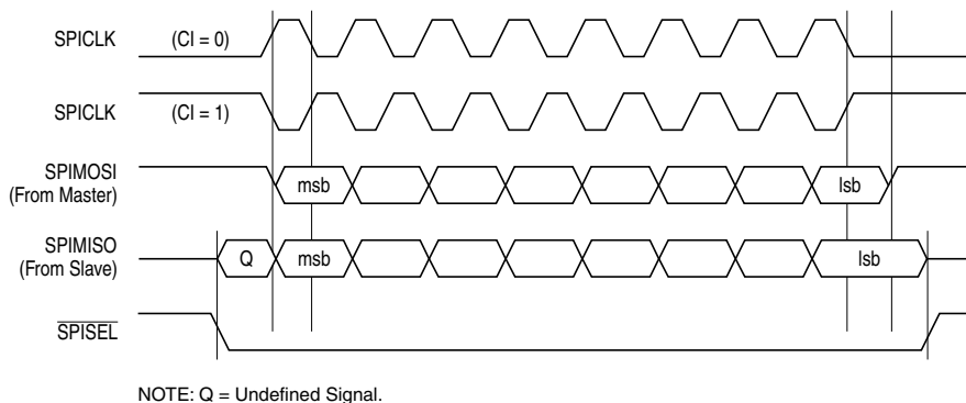
Figure 31-6. SPI Transfer Format with SPMODE[CP] = 1
