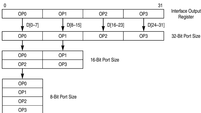
Figure 13-20. Interface to Different Port Size Devices
