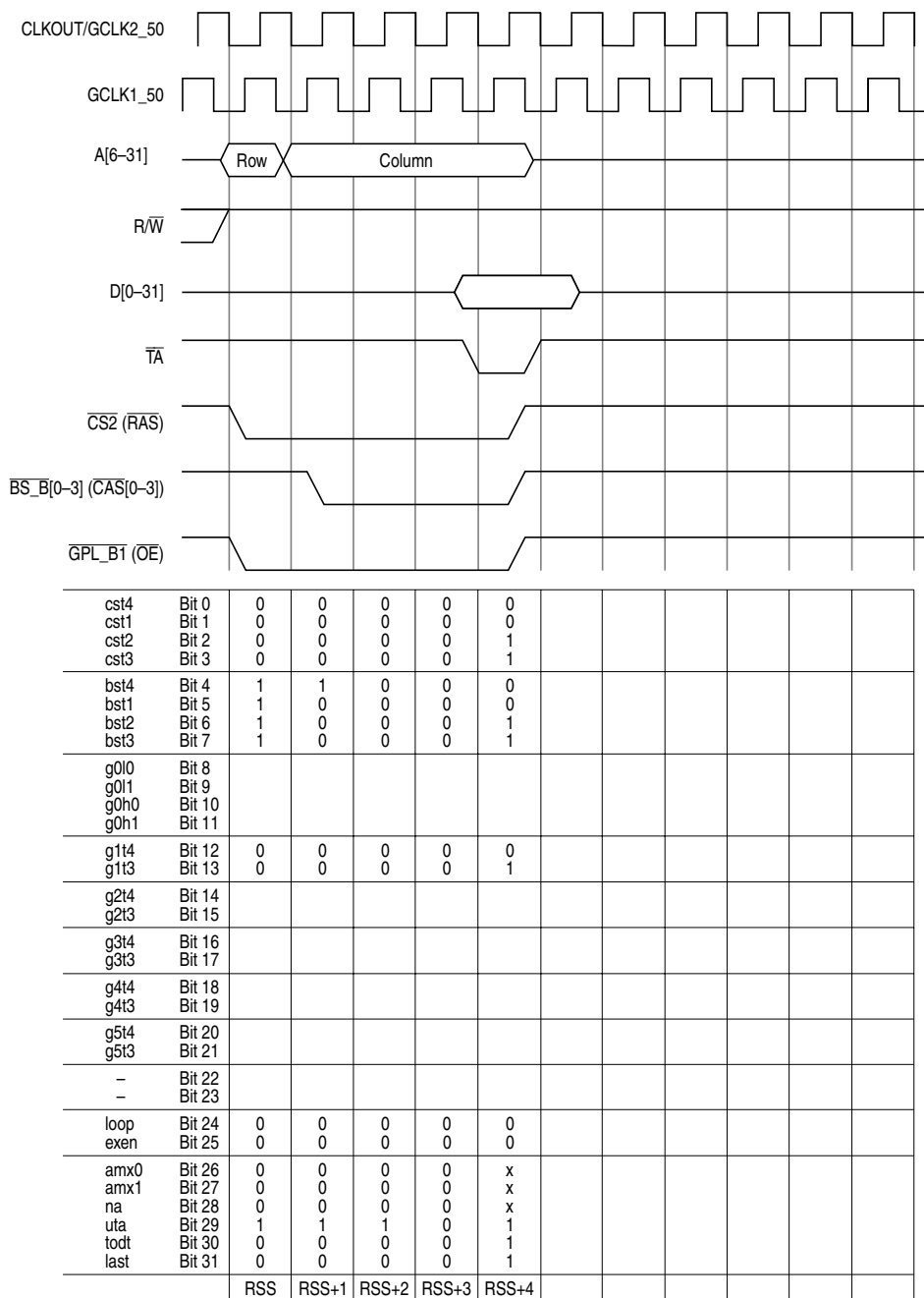
Figure 15-64. EDO DRAM Single-Beat Read Access
