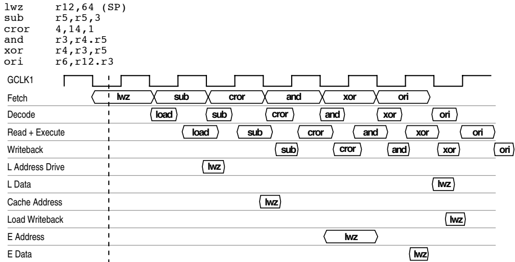
Figure 9-4. Private Writeback Bus Load Timing
