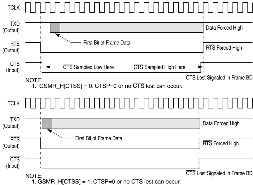
Figure 21-11. CTS Lost in Synchronous Protocols
