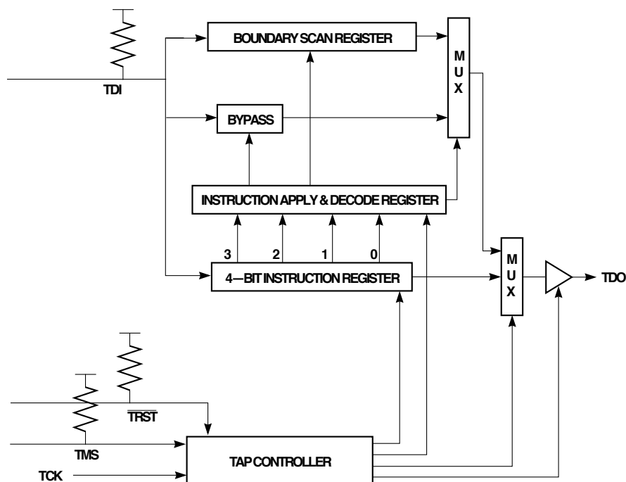
Figure 45-1. Test Logic Block Diagram
