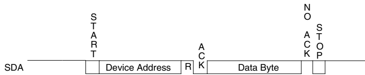
Figure 33-5. I 2 C Master Read Timing
