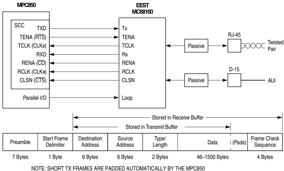
Figure 27-3. Connecting the MPC850 to Ethernet
