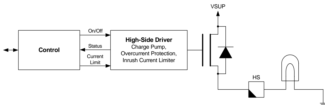
Figure 21. High-Side Circuitry
