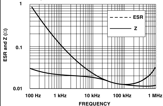
T97 1500 \mu\text{F} - 4 V 'R' CASE SIZE ESR and Z vs. FREQUENCY
