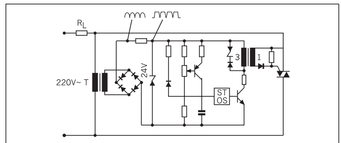
Triac phase angle control
