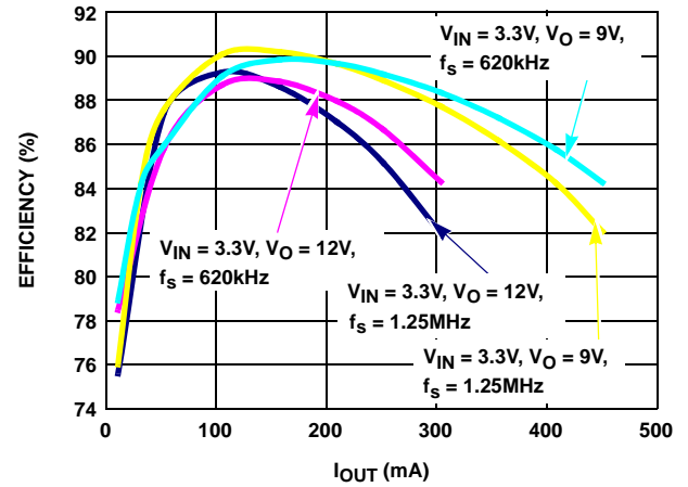
FIGURE 2. BOOST EFFICIENCY vs I_{OUT}
