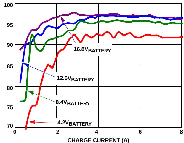
FIGURE 14. EFFICIENCY vs CHARGE CURRENT AND BATTERY VOLTAGE (EFFICIENCY \text{DC}_{\text{IN}} = 20\text{V} )
