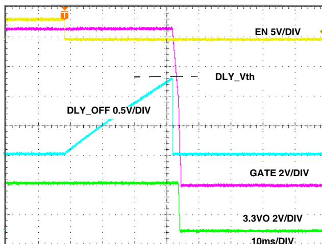
FIGURE 15. ISL8723 3.3V TURN-OFF
