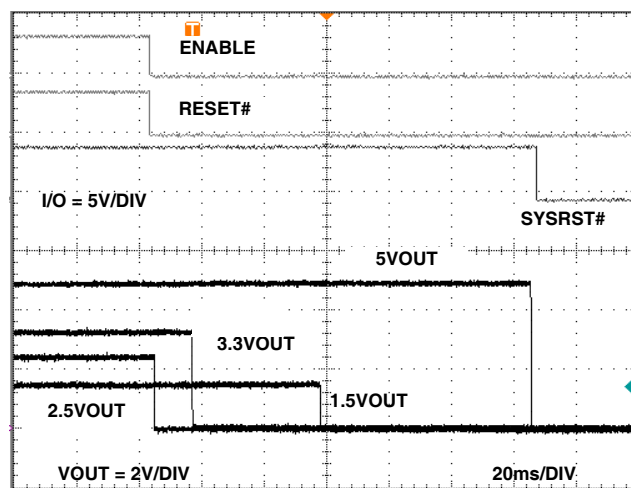
FIGURE 13. ISL8723 SEQUENCED TURN-OFF
