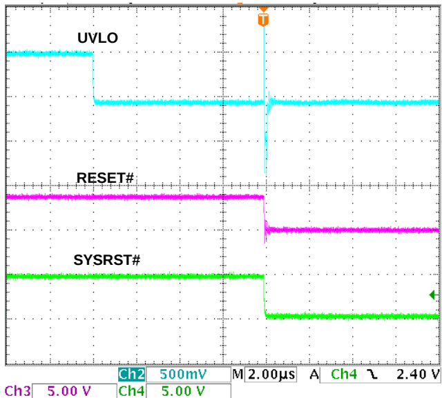
FIGURE 20. UVLO INVALID to RESET# and SYSRST# LOW
