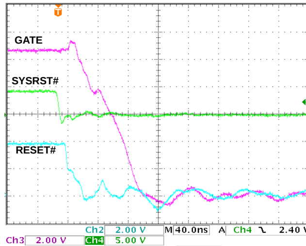
FIGURE 17. SYSRST# LOW to GATE and RESET# LOW
