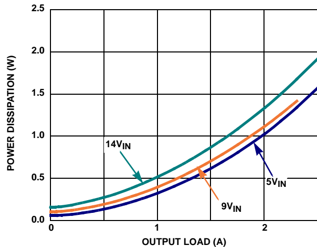
FIGURE 12. POWER DISSIPATION vs LOAD ( V_{OUT} = 1.5V , 500kHz)
