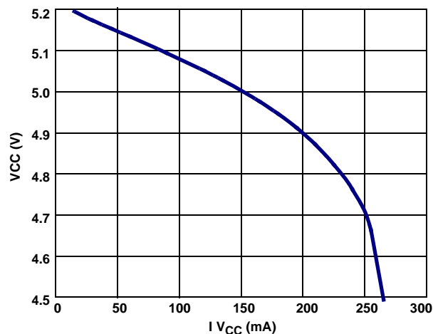
FIGURE 17. V_{CC} LOAD REGULATION
