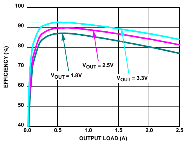
FIGURE 1. EFFICIENCY vs LOAD ( V_{IN} = 5V )
