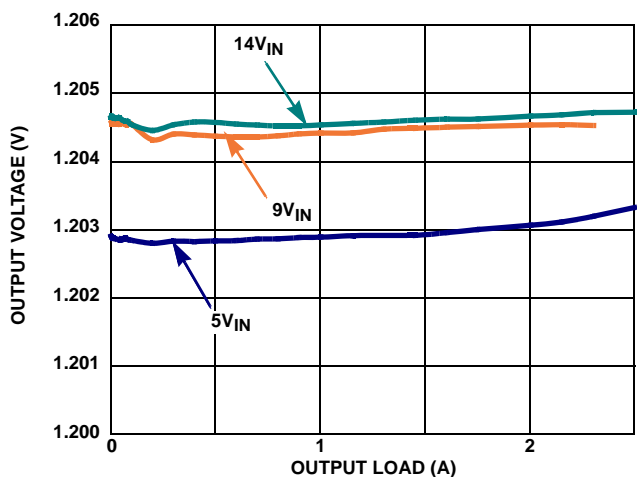
FIGURE 4. V_{OUT} REGULATION vs LOAD ( V_{OUT} = 1.2V , 500kHz)
