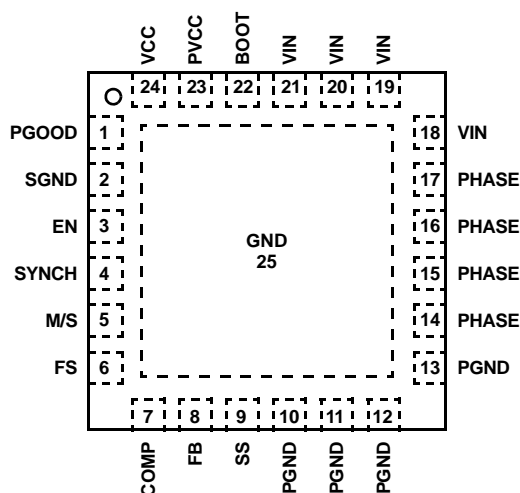
ISL8502 (24 LD QFN) TOP VIEW
