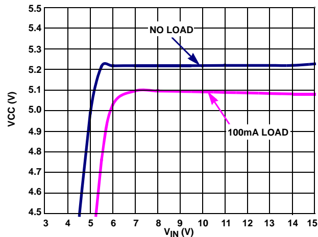
FIGURE 18. V_{CC} REGULATION vs V_{IN}
