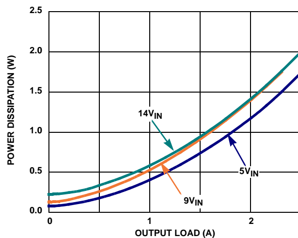
FIGURE 14. POWER DISSIPATION vs LOAD ( V_{OUT} = 2.5V , 500kHz)
