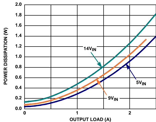
FIGURE 10. POWER DISSIPATION vs LOAD ( V_{OUT} = 0.6V , 500kHz)
