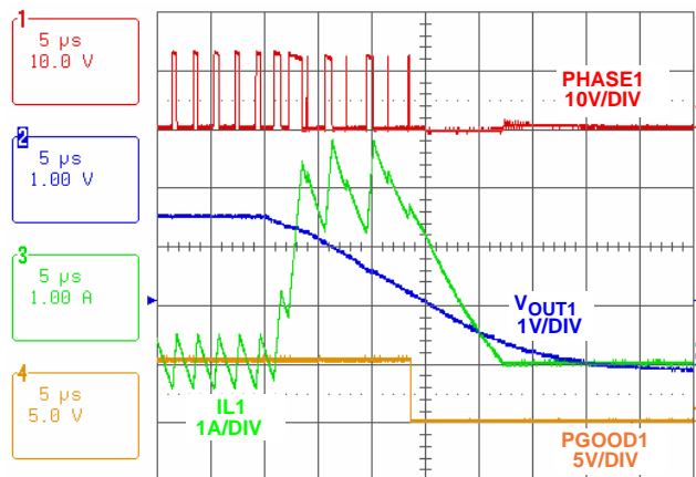
FIGURE 26. POSITIVE OUTPUT SHORT CIRCUIT
