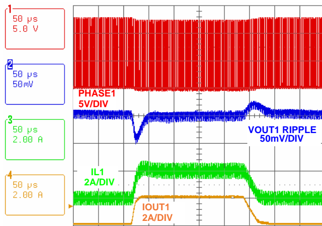
FIGURE 30. LOAD TRANSIENT
