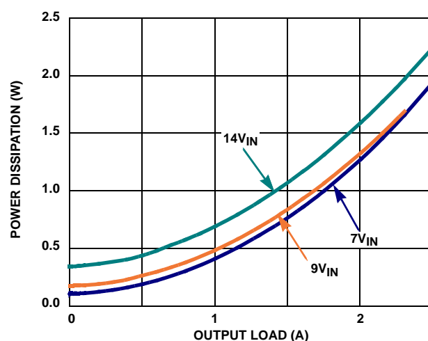
FIGURE 16. POWER DISSIPATION vs LOAD ( V_{OUT} = 5V , 500kHz)
