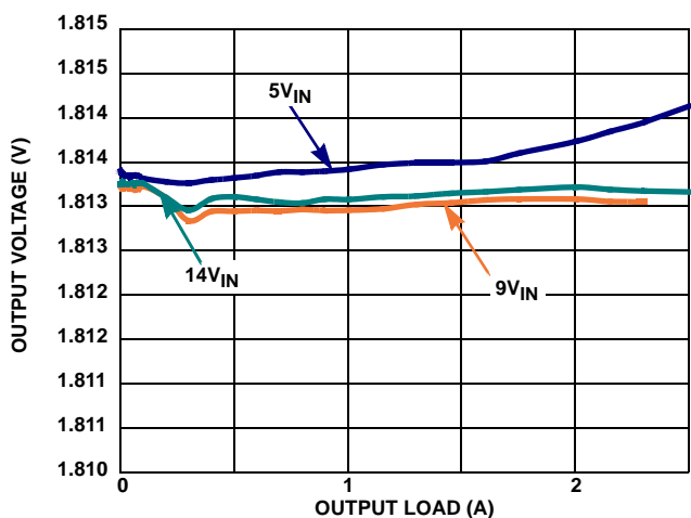
FIGURE 6. V_{OUT} REGULATION vs LOAD ( V_{OUT} = 1.8V , 500kHz)
