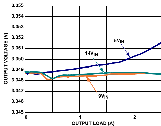
FIGURE 8. V_{OUT} REGULATION vs LOAD ( V_{OUT} = 3.3V , 500kHz)
