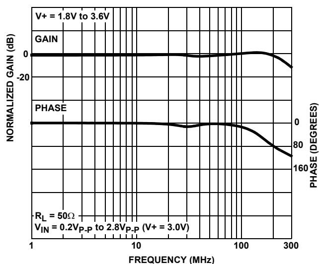
FIGURE 14. FREQUENCY RESPONSE
