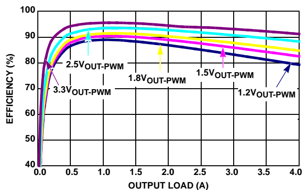
FIGURE 5. EFFICIENCY vs LOAD (1MHz 5 V_{\text{IN}} PWM)
