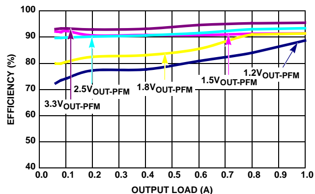
FIGURE 6. EFFICIENCY vs LOAD (1MHz 5 V_{\text{IN}} PFM)
