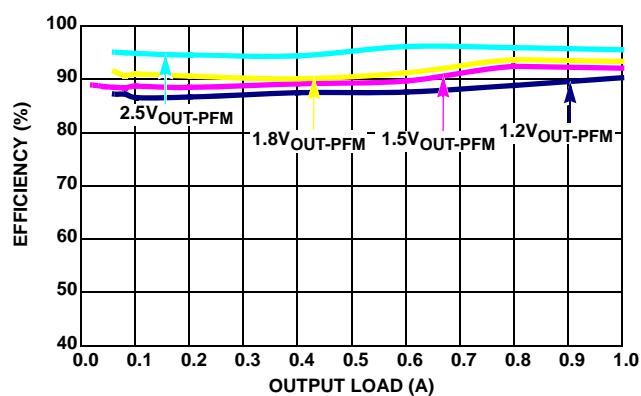
FIGURE 4. EFFICIENCY vs LOAD (1MHz 3.3 V_{\text{IN}} PFM)
