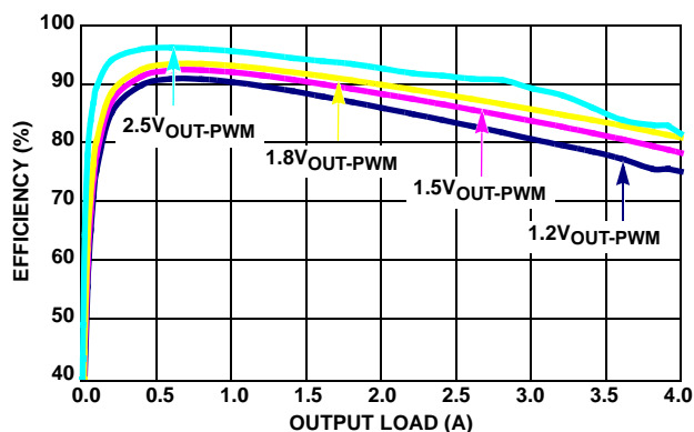
FIGURE 3. EFFICIENCY vs LOAD (1MHz 3.3 V_{\text{IN}} PWM)
