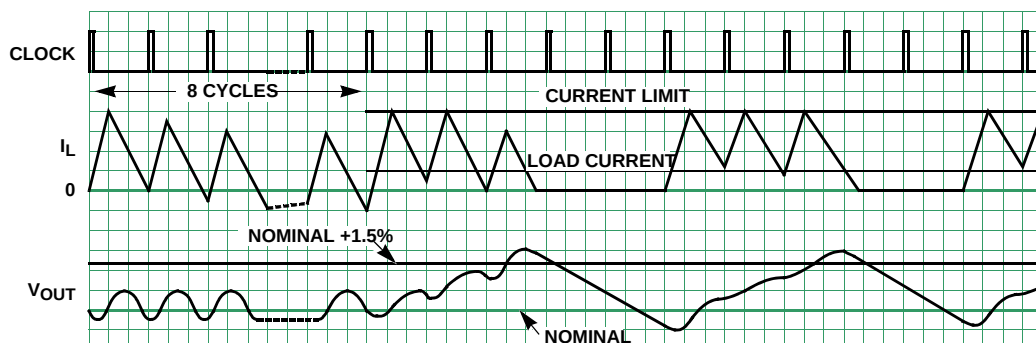
FIGURE 37. SKIP MODE OPERATION WAVEFORMS
