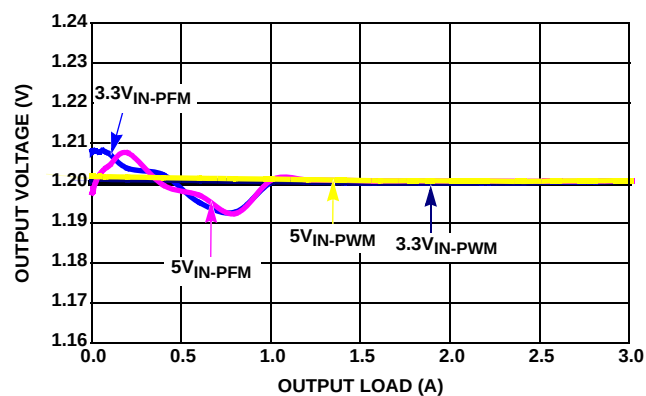
FIGURE 10. V_{OUT} REGULATION vs LOAD (1MHz, V_{OUT} = 1.2\text{V} )
