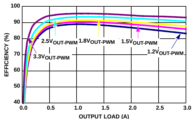
FIGURE 5. EFFICIENCY vs LOAD (1MHz 5V V_{IN} PWM)
