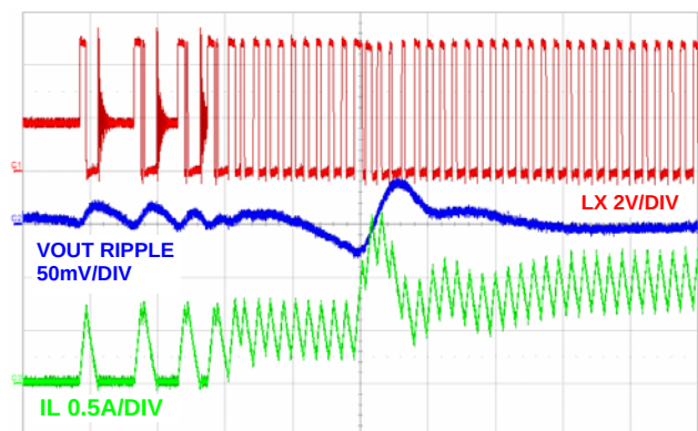
FIGURE 19. MODE TRANSITION DCM TO CCM, (50μs/DIV)
