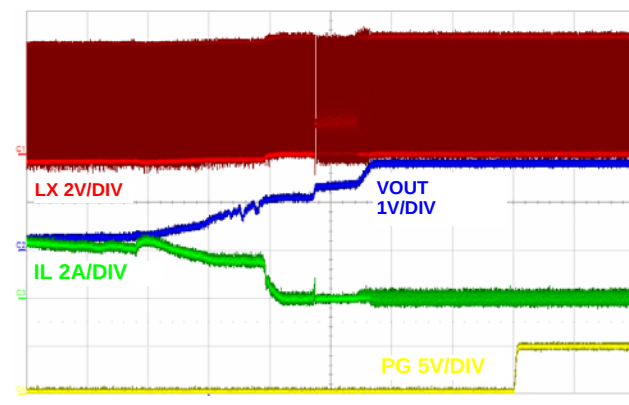
FIGURE 30. OUTPUT SHORT CIRCUIT RECOVERY, (500µs/DIV)
