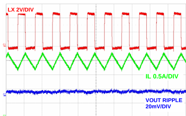
FIGURE 17. STEADY STATE OPERATION WITH FULL LOAD, (5μs/DIV)
