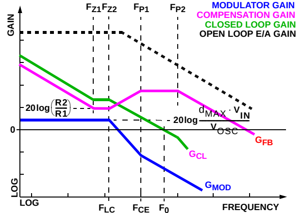
FIGURE 25. ASYMPTOTIC BODE PLOT OF CONVERTER GAIN
