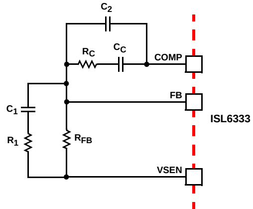
FIGURE 17. COMPENSATION CIRCUIT
