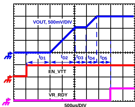
FIGURE 9. SOFT-START WAVEFORMS
