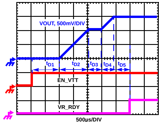
FIGURE 9. SOFT-START WAVEFORMS
