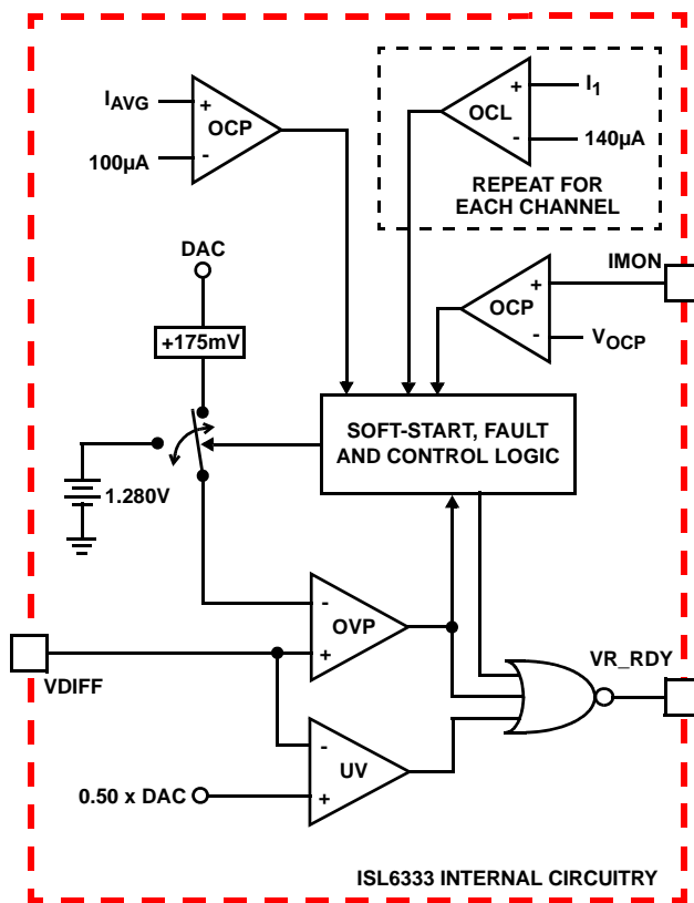
FIGURE 18. POWER GOOD AND PROTECTION CIRCUITRY
