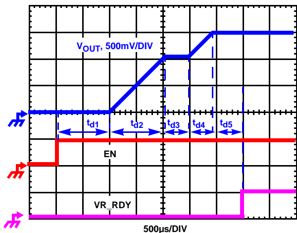
FIGURE 16. SOFT-START WAVEFORMS
