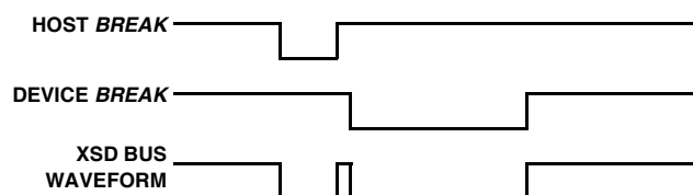
FIGURE 4B. WHEN THE HOST POWER-ON BREAK IS NARROWER THAN 60μs
