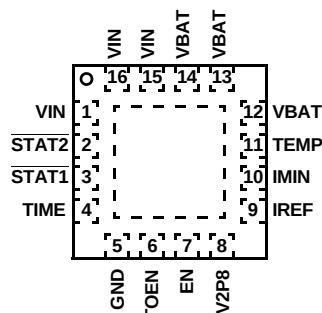
ISL6292D (16 LEAD QFN) TOP VIEW
