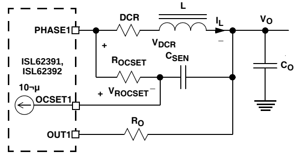
FIGURE 26. OVERCURRENT-SET CIRCUIT
