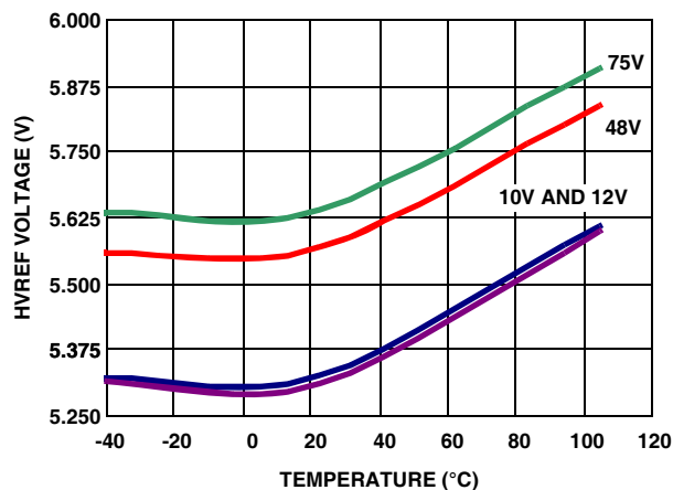
FIGURE 9. HVREF VOLTAGE
