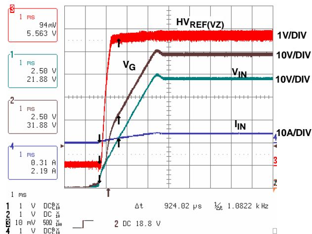
FIGURE 10. FIRST SUPPLY START-UP
