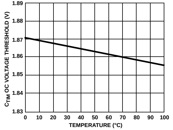
FIGURE 6. C TIM OC VOLTAGE THRESHOLD
