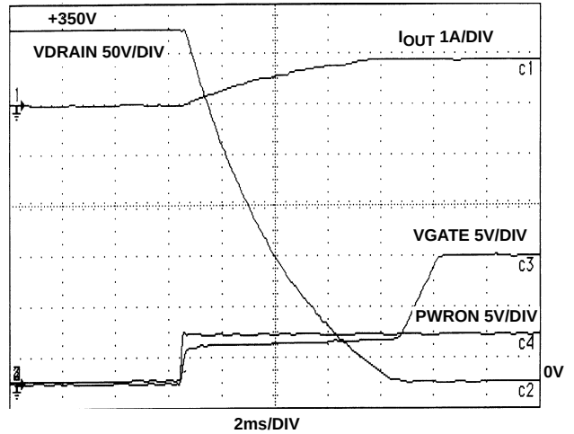
FIGURE 20. +350V LOW SIDE SWITCHING C_{GATE} = 1000\text{pF}
