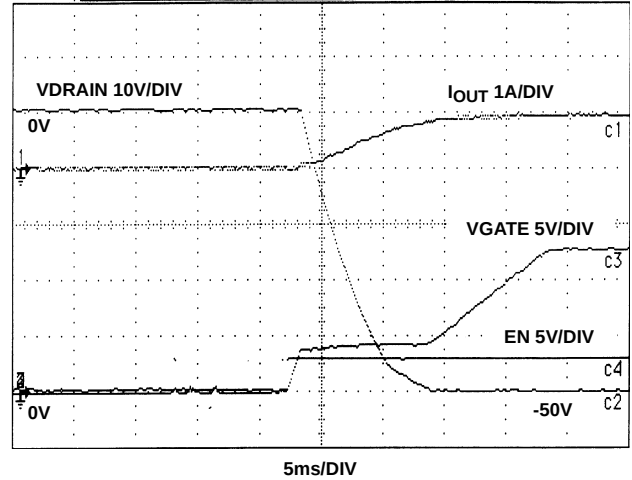
FIGURE 18. -50V LOW SIDE SWITCHING C_{GATE} = 1000\text{pF}
