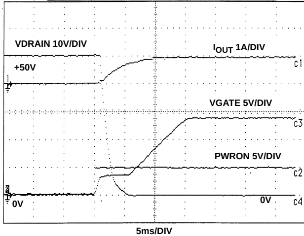
FIGURE 17. +50V LOW SIDE SWITCHING C_{GATE} = 100\text{pF}
