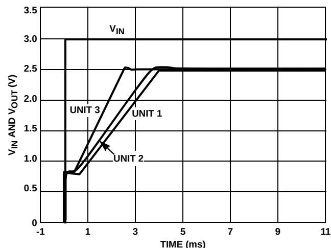
FIGURE 119. TURN-ON TIME
