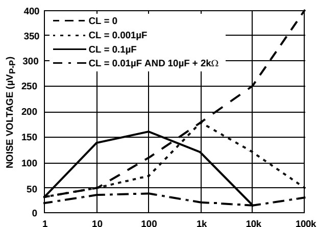
FIGURE 117. NOISE REDUCTION
