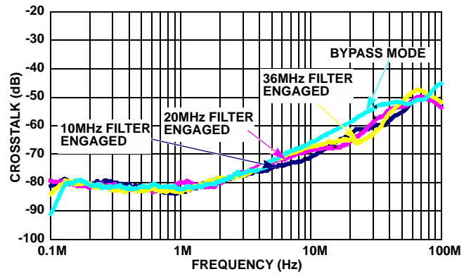
FIGURE 26. INTRA-CHANNEL CROSSTALK: COMPONENT INPUT TO S-VIDEO OUTPUT
