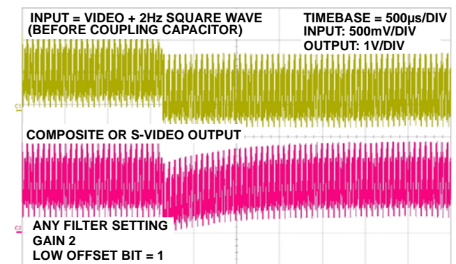
FIGURE 28. COMPOSITE/S-VIDEO: CLAMP RESPONSE TO +250mV STEP ON INPUT (LOW OFFSET MODE)
