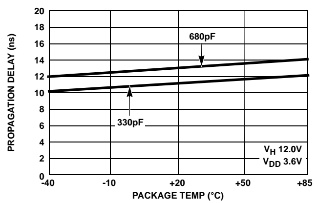
FIGURE 18. tp_{dL} vs TEMPERATURE
