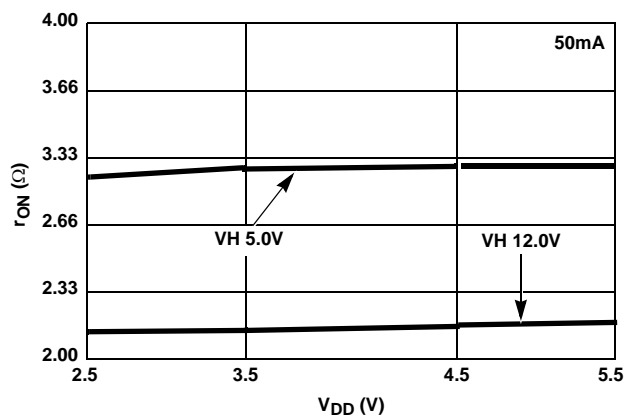
FIGURE 6. r_{ON} vs V_{DD} SINK RESISTANCE
