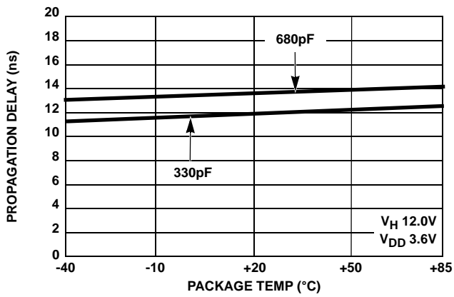
FIGURE 17. tp_{dL} vs TEMPERATURE
