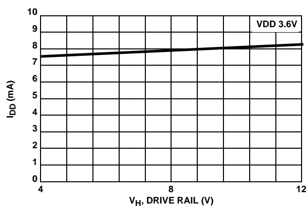
FIGURE 8. I_{DD} vs V_H @ 50MHz (NO LOAD)
