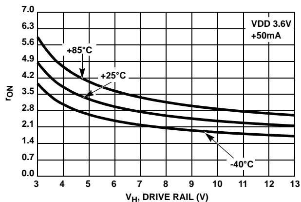
FIGURE 4. DRIVER r_{ON} vs V_H SINK RESISTANCE
