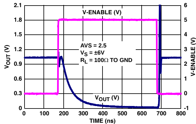
FIGURE 17. ENABLE TO OUTPUT DELAY
