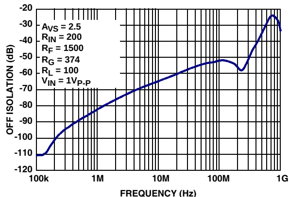
FIGURE 11. INPUT OFF ISOLATION GAIN vs FREQUENCY SINGLE-ENDED
