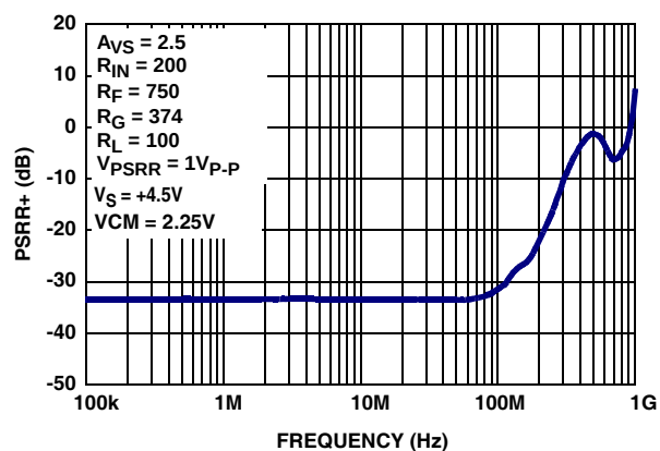
FIGURE 10. PSRR+ vs FREQUENCY vs V_S (SINGLE SUPPLY)
