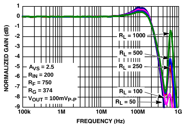
FIGURE 1. SINGLE-ENDED GAIN vs FREQUENCY vs R_L
