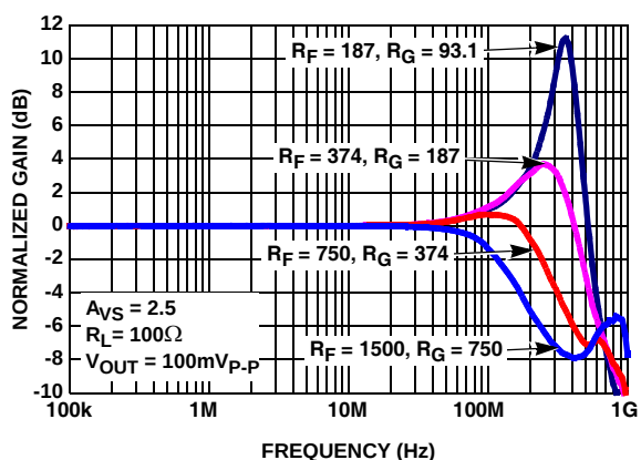
FIGURE 5. SINGLE-ENDED GAIN vs FREQUENCY vs R_F/R_G
