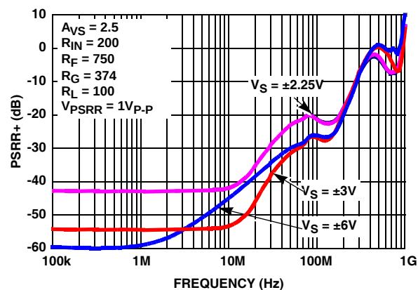
FIGURE 8. PSRR+ vs FREQUENCY vs V_S (DUAL SUPPLIES)
