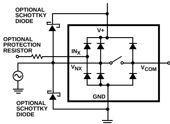
FIGURE 9. OVERVOLTAGE PROTECTION
