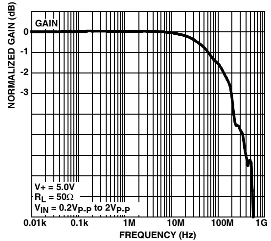
FIGURE 14. FREQUENCY RESPONSE
