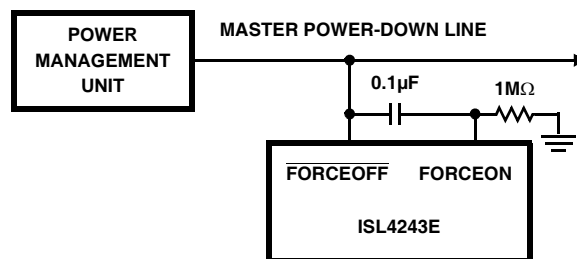
With any of the previous mentioned control schemes, the time required to exit power-down, and resume transmission is only 100 \mu s. A mouse, or other application, may need more time to wake up from shutdown. If automatic power-down is being utilized, the RS-232 device will reenter power-down if valid receiver levels aren't reestablished within 30 \mu s of the ISL4243E powering up. Figure 5 illustrates a circuit that keeps the ISL4243E from initiating automatic power-down for 100ms after powering up. This gives the slow-to-wake peripheral circuit time to reestablish valid RS-232 output levels.
