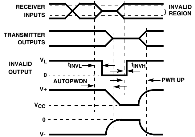
FIGURE 11. AUTOMATIC POWERDOWN AND \overline{INVALID} TIMING DIAGRAM
