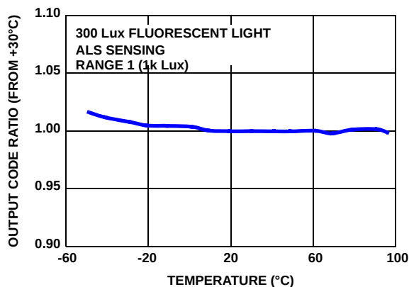
FIGURE 12. OUTPUT CODE vs TEMPERATURE
