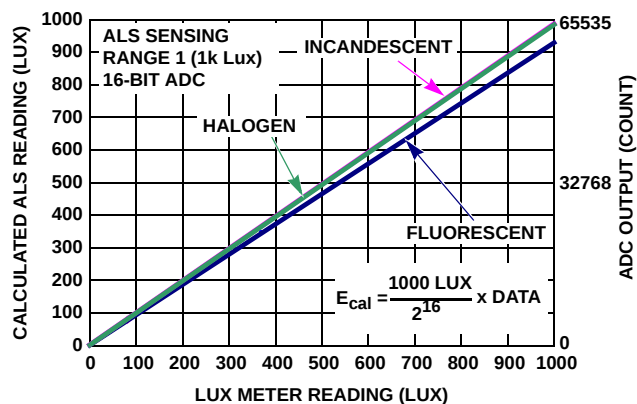
FIGURE 10. SENSITIVITY TO FOUR LIGHT SOURCES
