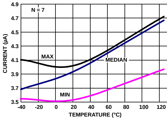
FIGURE 17. ISL28276 SUPPLY CURRENT vs TEMPERATURE, V_+, V_- = \pm 2.5V DISABLED, R_L = \text{INF}
