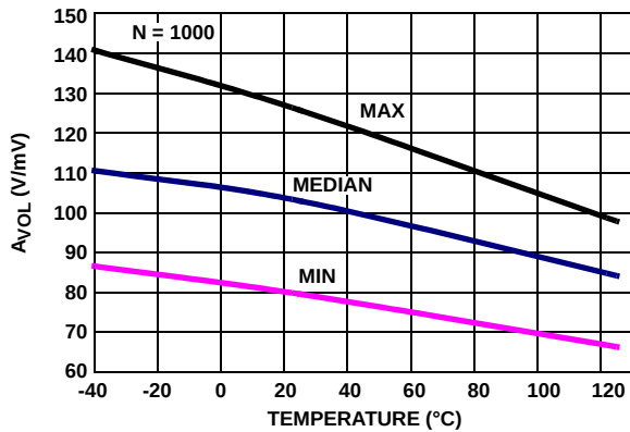
FIGURE 29. A_{VOL} vs TEMPERATURE, V_+, V_- = \pm 2.5V , R_L = 1k
