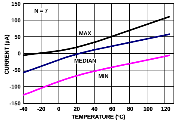
FIGURE 16. ISL28276 SUPPLY CURRENT vs TEMPERATURE, V_+, V_- = \pm 2.5V ENABLED, R_L = \text{INF}
