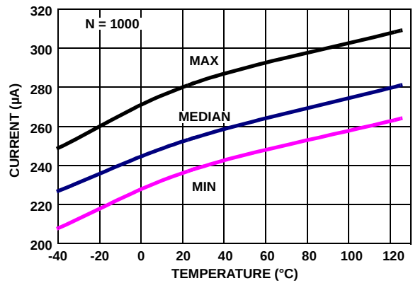
FIGURE 18. ISL28476 SUPPLY CURRENT vs TEMPERATURE, V_+, V_- = \pm 2.5V R_L = \text{INF}
