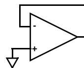
FIGURE 42. PREVENTING OSCILLATIONS IN UNUSED CHANNELS
