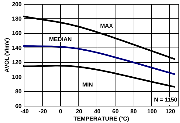
FIGURE 35. AVOL vs TEMPERATURE, V_+ = 5V , V_- = 0V , V_{CM} = 2.5V , R_L = 1k
