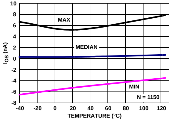
FIGURE 30. I_{OS} vs TEMPERATURE, V_+ = 5V , V_- = 0V , V_{CM} = 2.5V , R_L = \text{Open}
