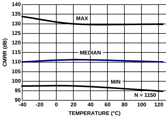
FIGURE 32. CMRR vs TEMPERATURE, V_{CM} = -2.5V TO +2.5V , V_+ = 5V , V_- = 0V
