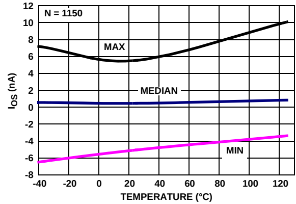
FIGURE 31. I_{OS} vs TEMPERATURE, V_+ = 5V , V_- = 0V , V_{CM} = 2.5V , R_L = \text{Open}
