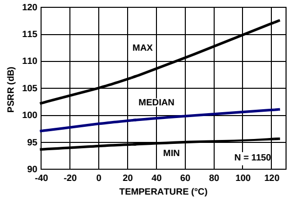
FIGURE 33. PSRR vs TEMPERATURE, V_+ = 5V , V_- = 0V , V_{CM} = 2.5V , R_L = \text{Open}
