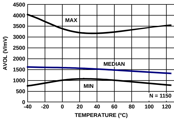
FIGURE 34. AVOL vs TEMPERATURE, V_+ = 5V , V_- = 0V , V_{CM} = 2.5V , R_L = 100k
