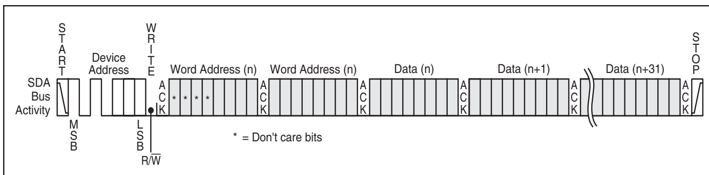
Figure 7. Page Write
