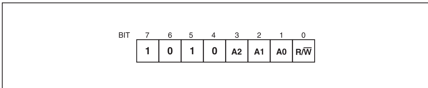
Figure 5. Slave Address
