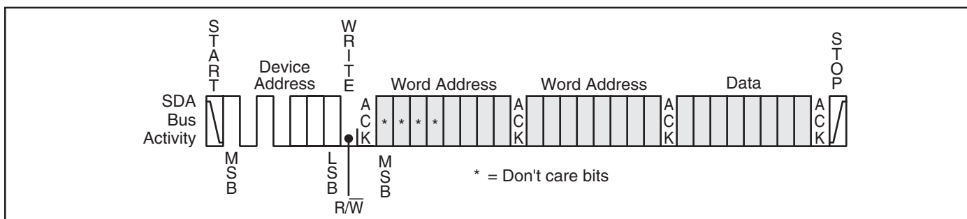
Figure 6. Byte Write
