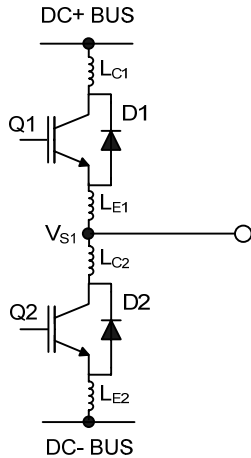
Figure 17: Parasitic Elements
