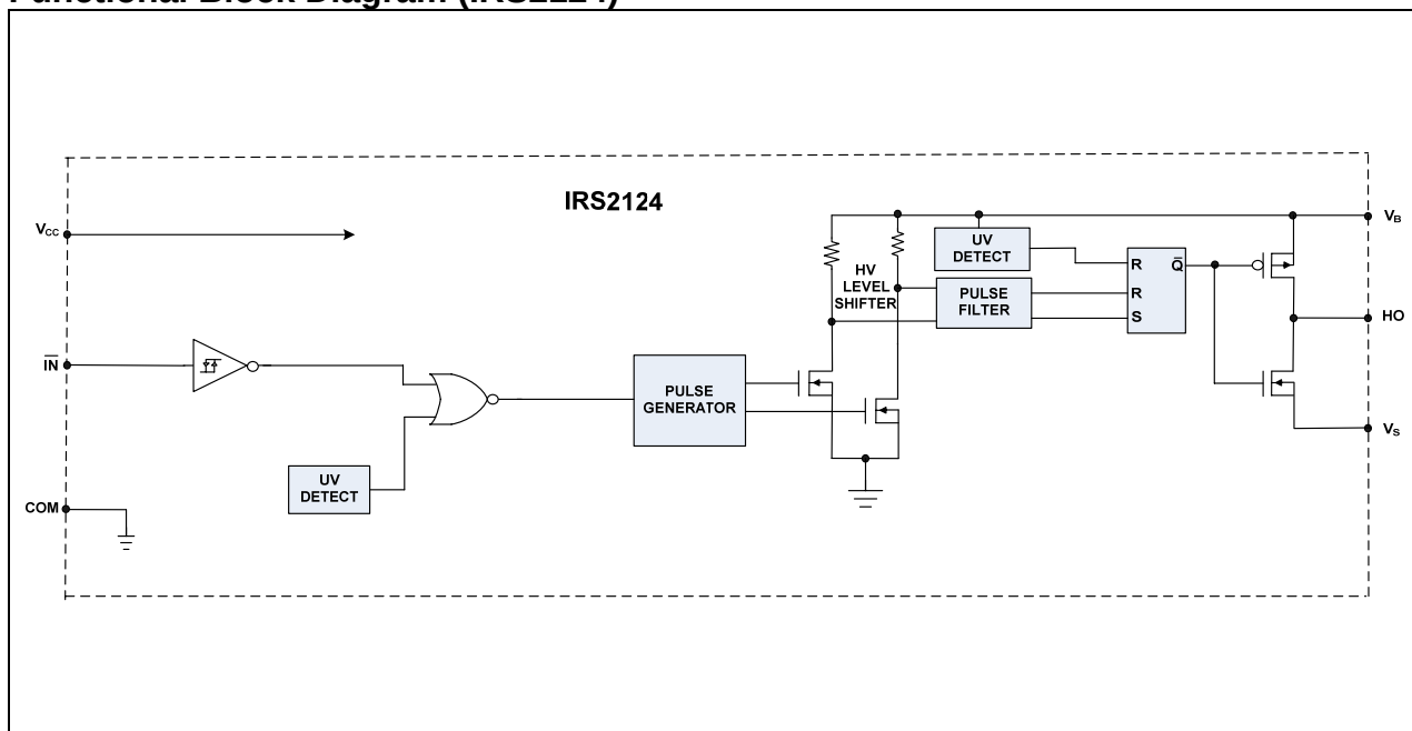
Functional Block Diagram (IRS2124)
