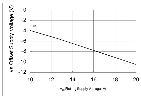
Figure 13. Maximum VS Negative Offset vs. Supply Voltage
