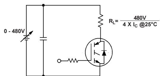
Fig. 20 - Pulsed Collector Current Test Circuit
