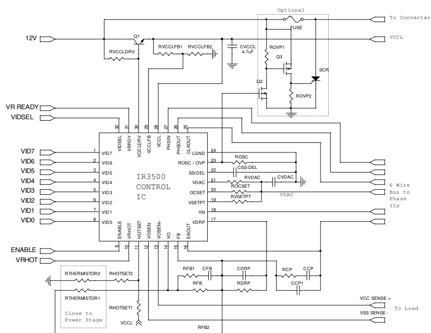
Figure 1 – Application Circuit
