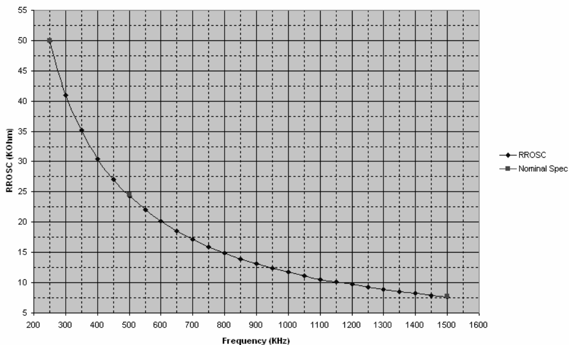
Figure 23 - Frequency variation with ROSC.
