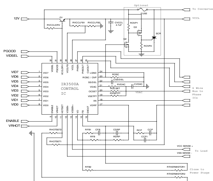
Figure 1 – Application Circuit
