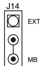
Figure 5: Jumper Setting to Power Up from a Host Board
