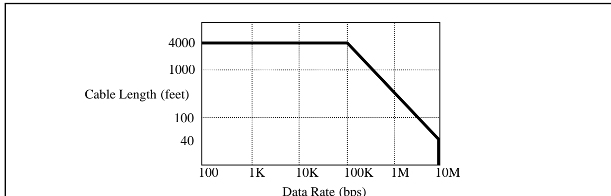
Figure 3. Cable Length vs. Data Rate (30% jitter).
