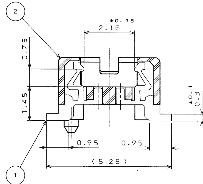
SECT. A-A (SCALE 10:1)
