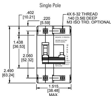
Panel Mounting Details Single Pole
