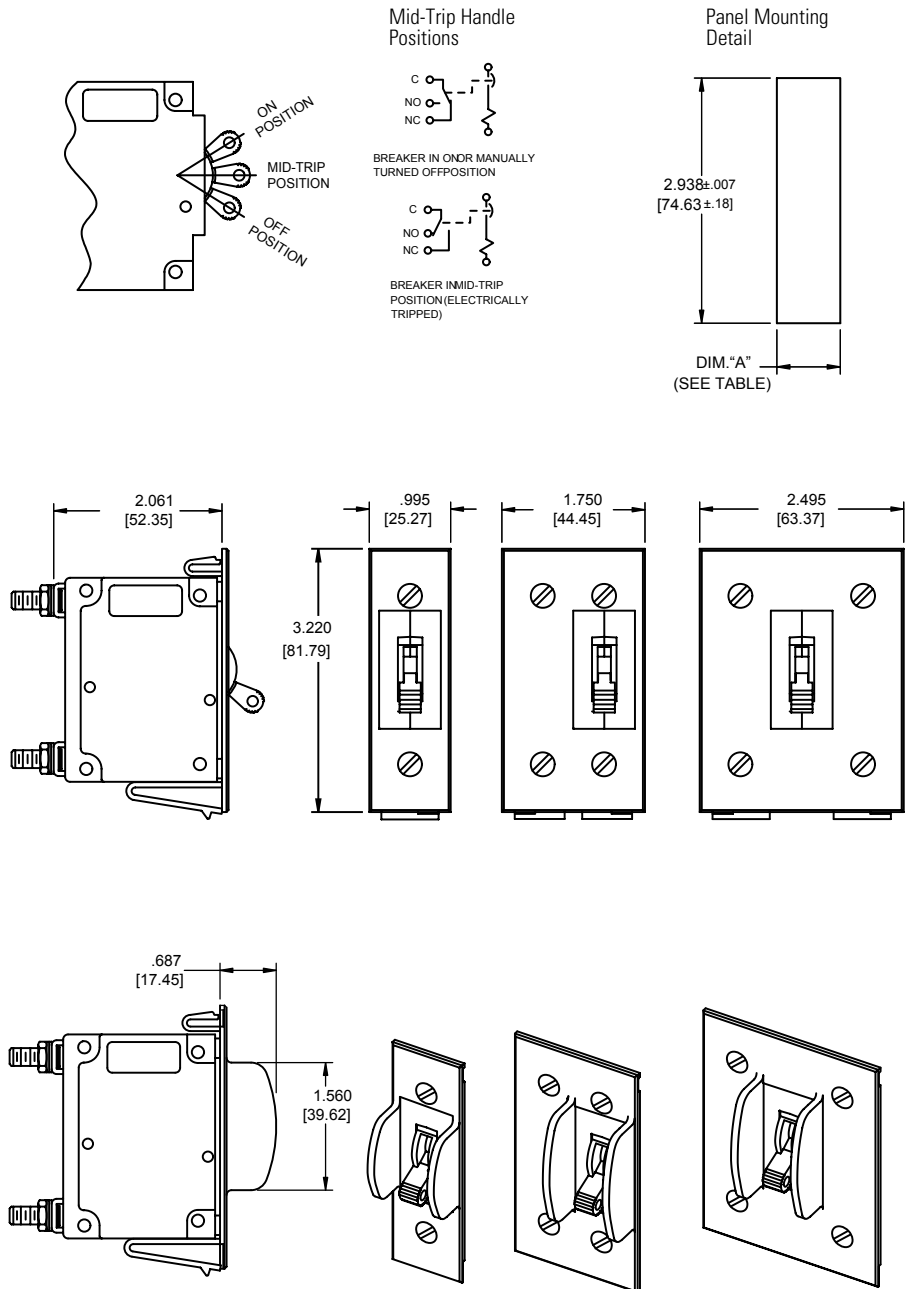
Panel Mounting Options
