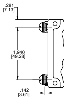
Screw Terminal
