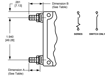
Series with Auxiliary Switch
