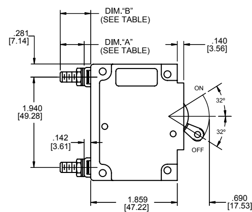
Two Pole
