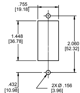
Bullet Terminal
