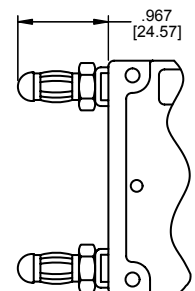
Bullet Terminal
