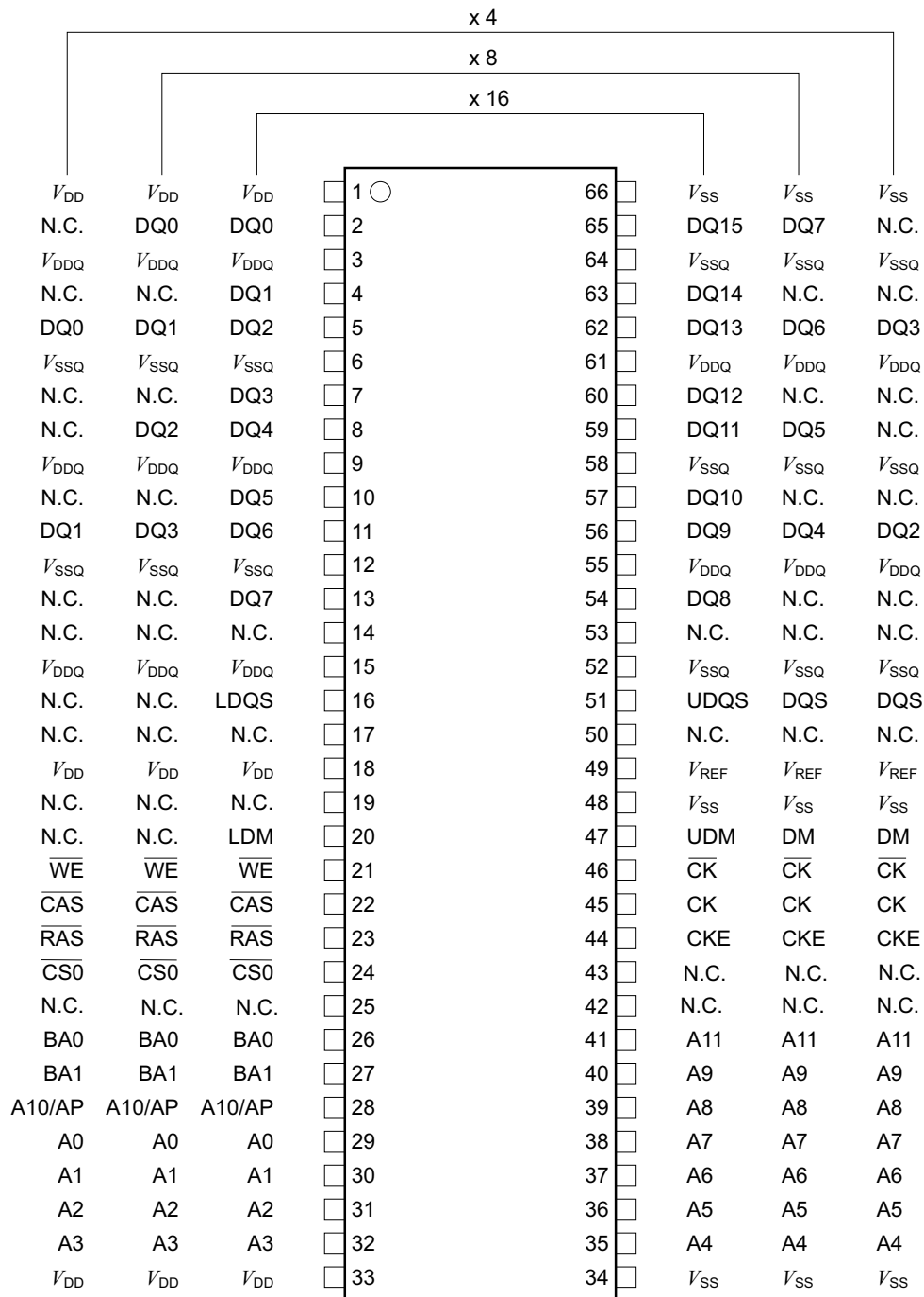
FIGURE 4 Pin Configuration TSOP1-66
