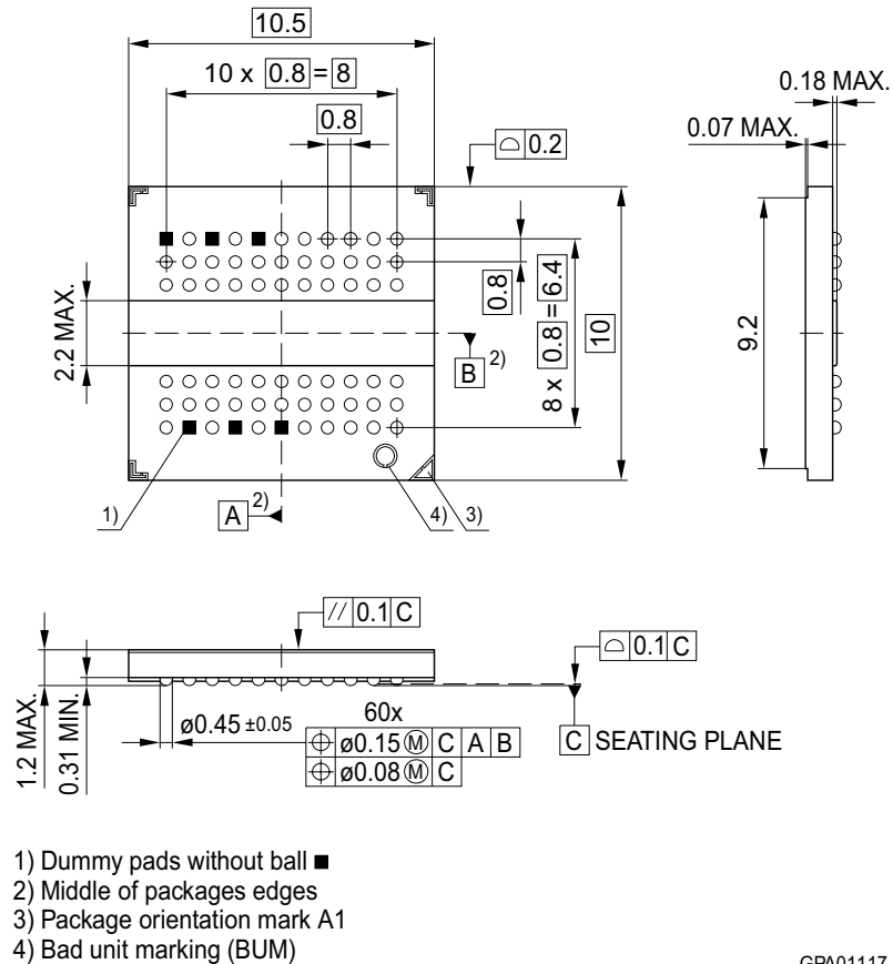
FIGURE 13 Package Outline P(G)-TFBGA-60-6
