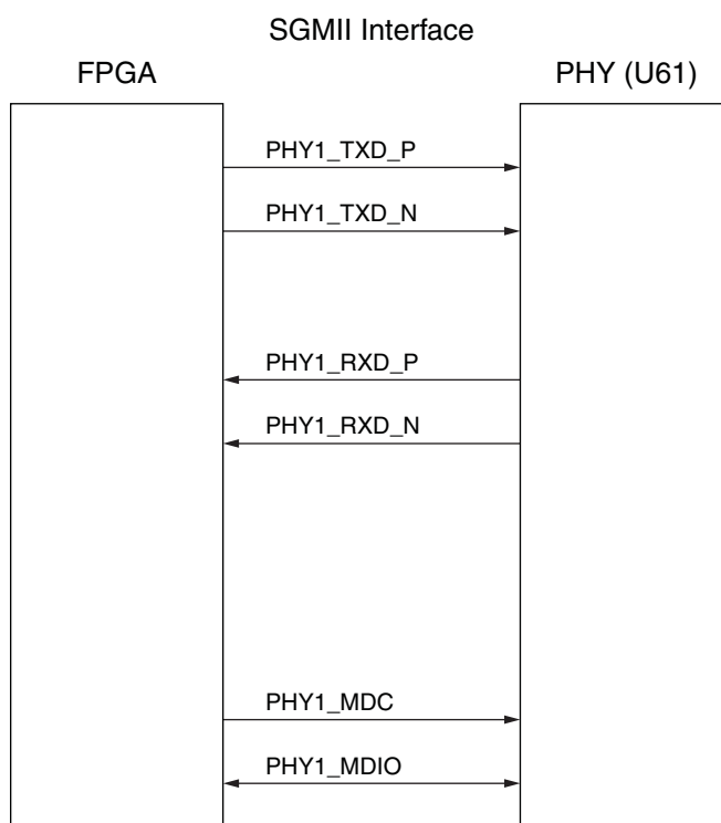
Figure 2-9: SGMII Interface
