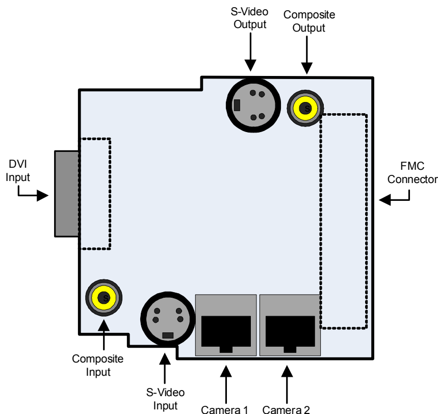
Figure 2-2: Port Diagram
