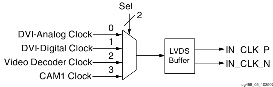
Figure 2-5: Clock Routing
