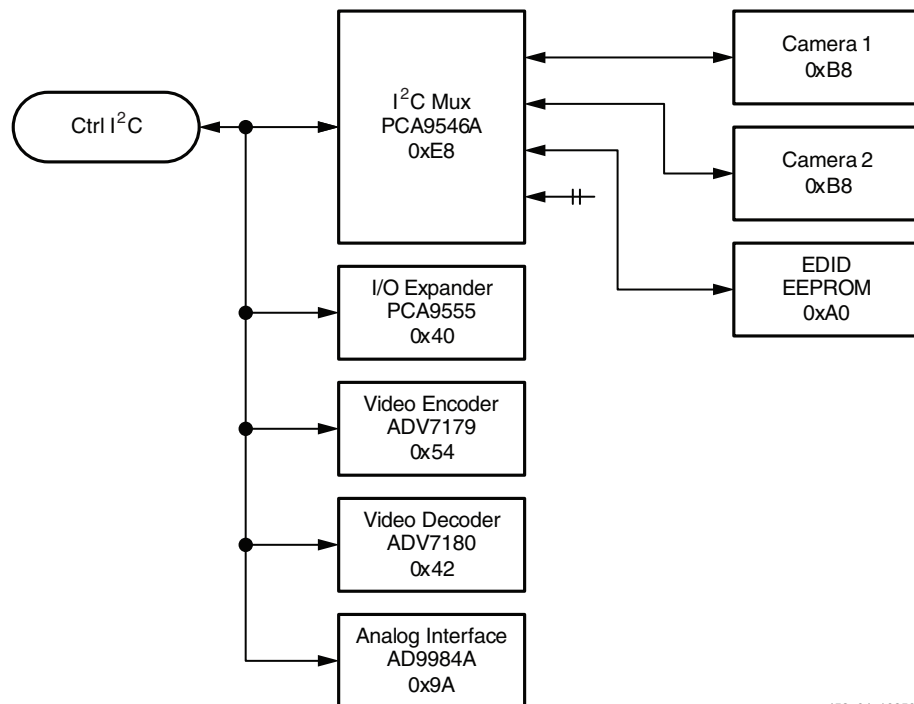
Figure 2-4: Control I2C Bus
