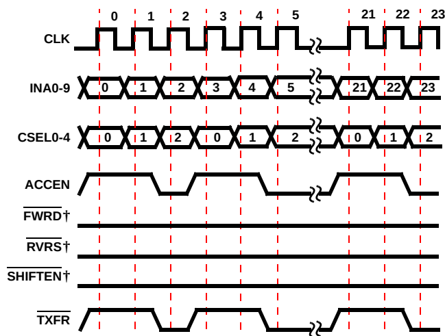
FIGURE 18. CONTROL SIGNAL TIMING FOR 24-TAP DECIMATE X3 FILTER
