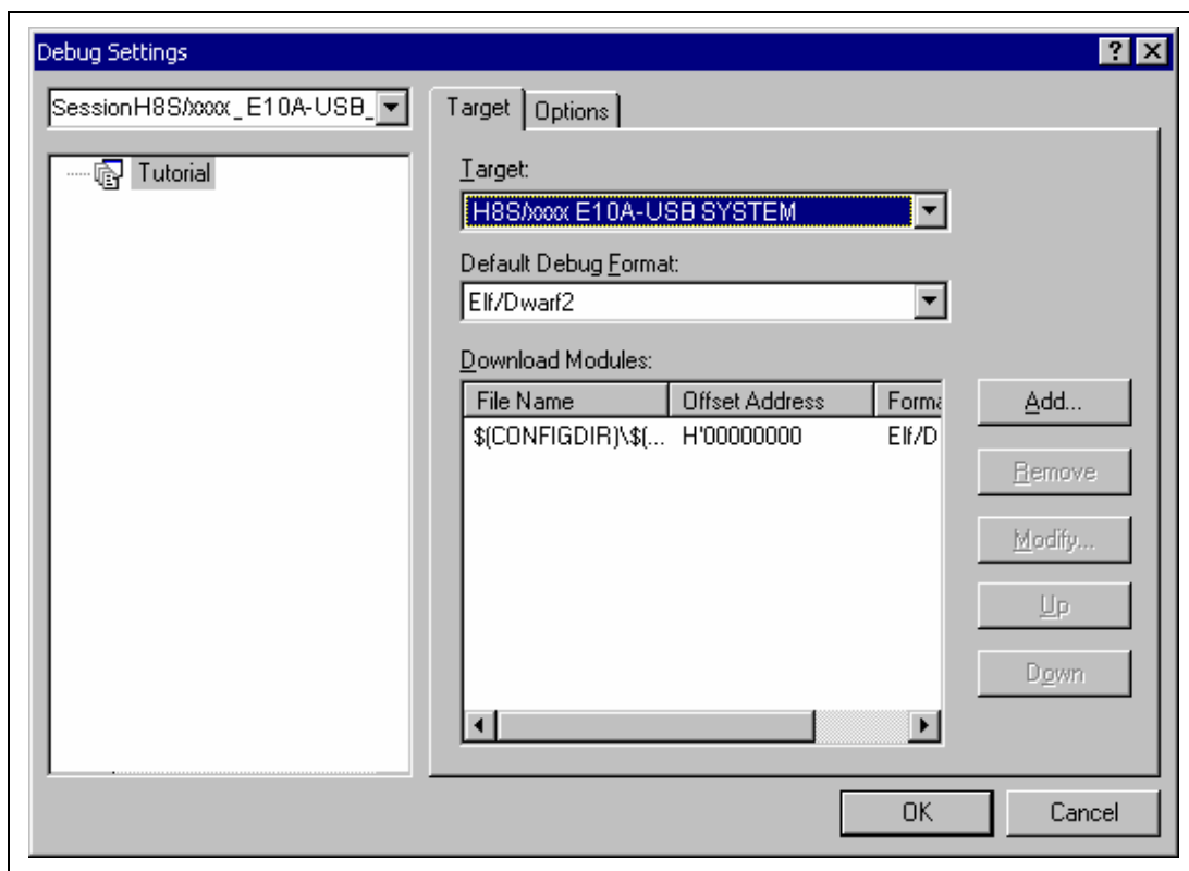
Figure 4.13 [Debug Settings] Dialog Box ([Target] Page)
