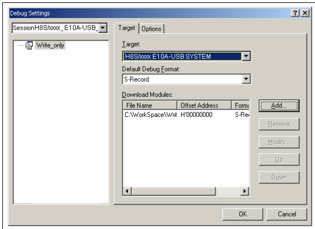
Figure 4.23 [Debug Settings] Dialog Box ([Target] Page)
