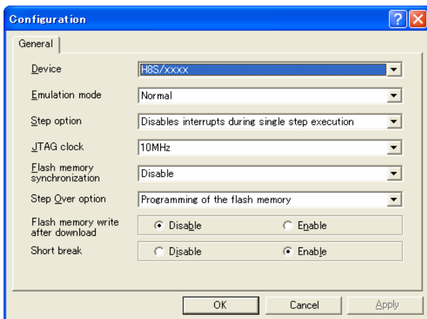
Figure 5.1 [Configuration] Dialog Box ([General] Page)
