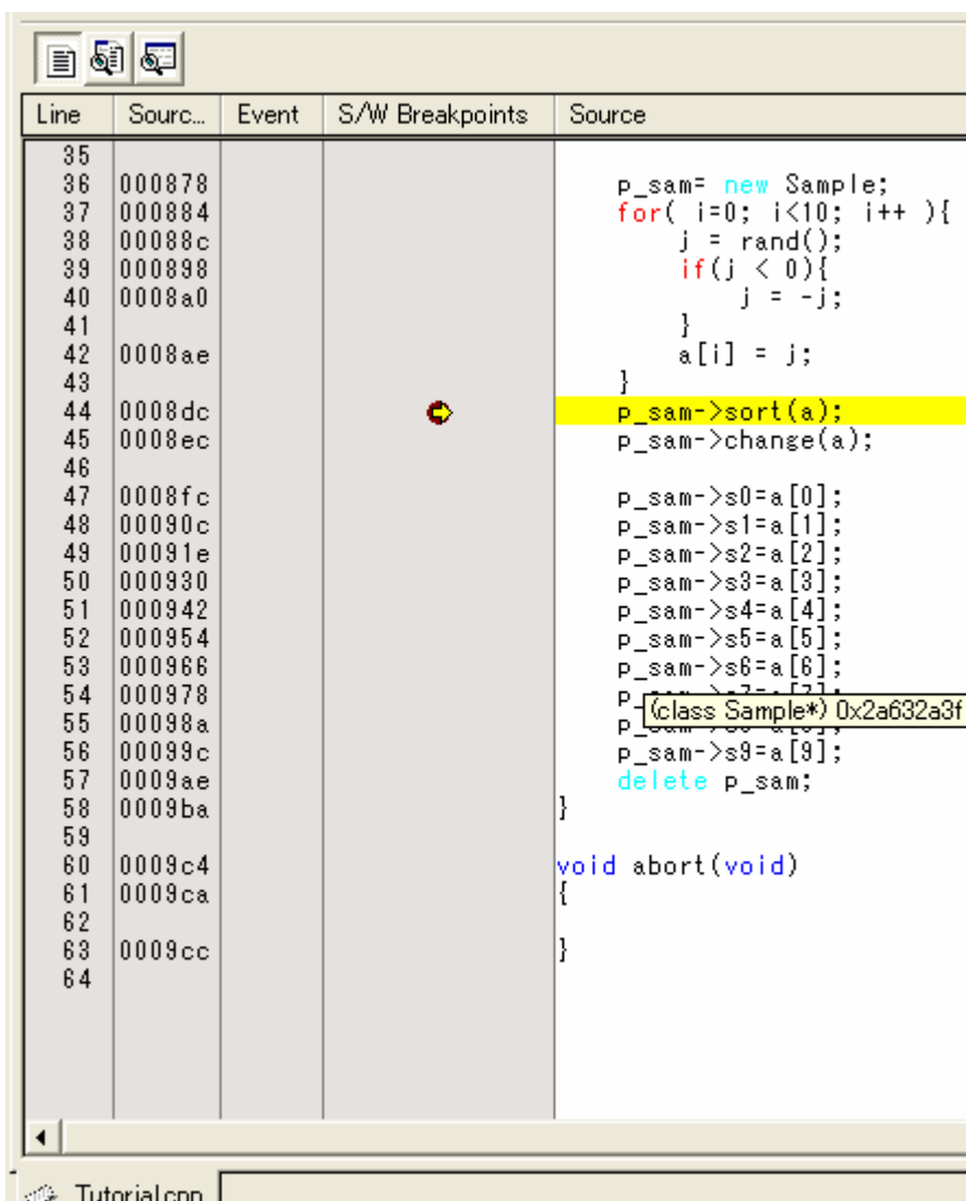
Figure 6.10 [Editor] Window (Break State)
