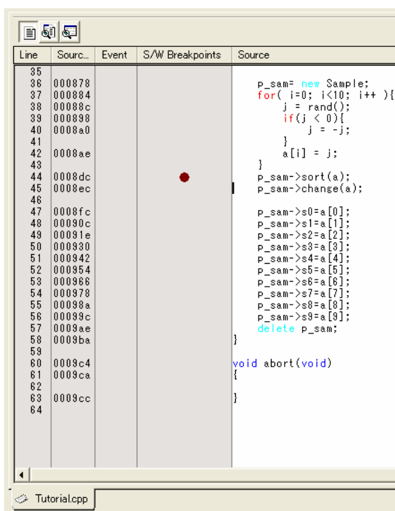
Figure 6.6 [Editor] Window (Setting a PC Breakpoint)
