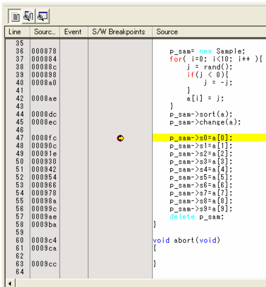
Figure 6.33 [Editor] Window at Execution Stop (PC Break)
